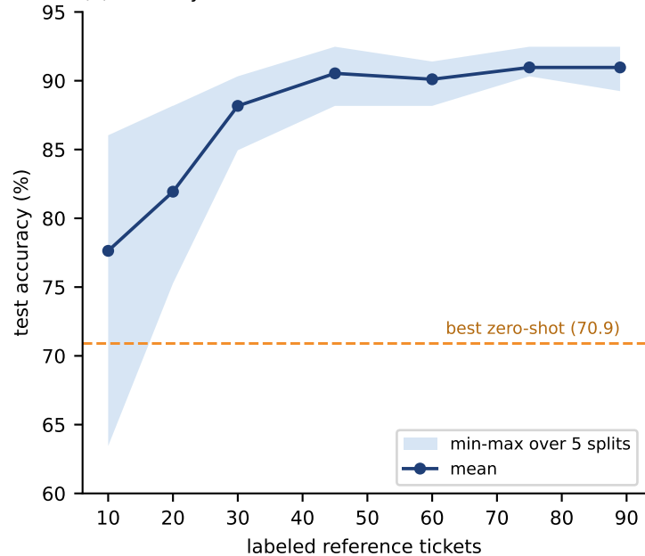
(b) accuracy vs. reference-set size
