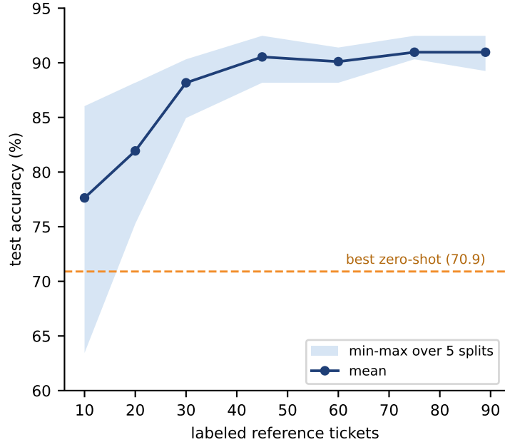
(b) accuracy vs. reference-set size
