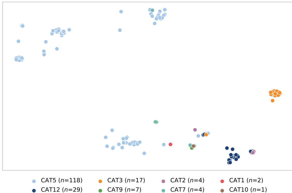
(a) ticket embedding space (t-SNE)
