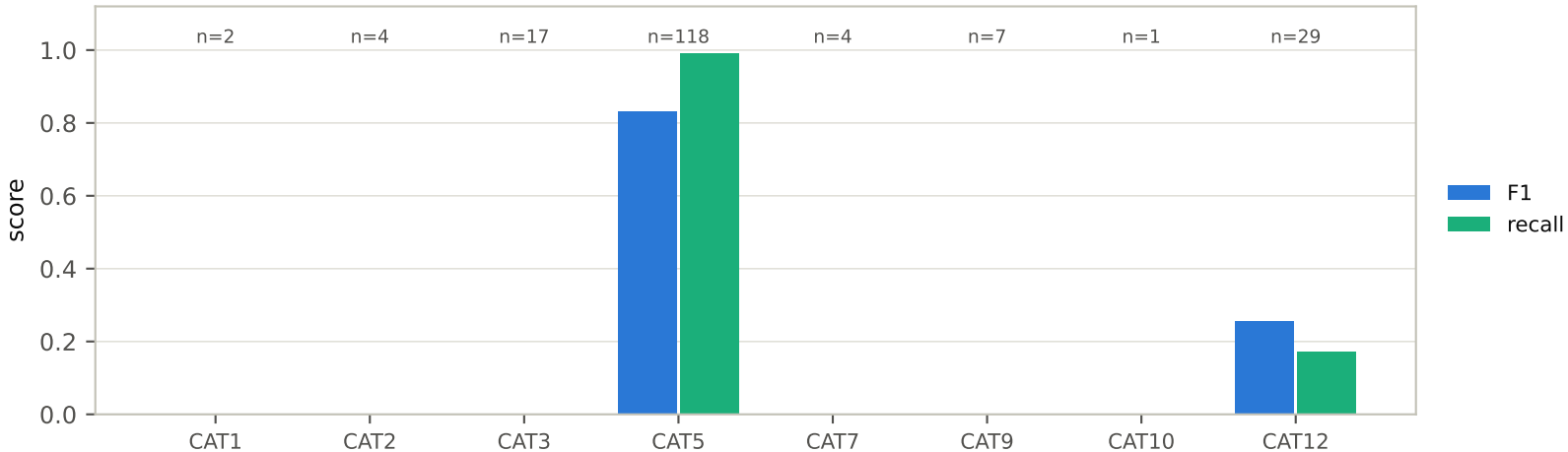
Per-class metrics, best run (gliclass-modern-base-v3.0__en-event)
