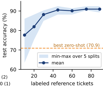
(b) accuracy vs. reference-set size
