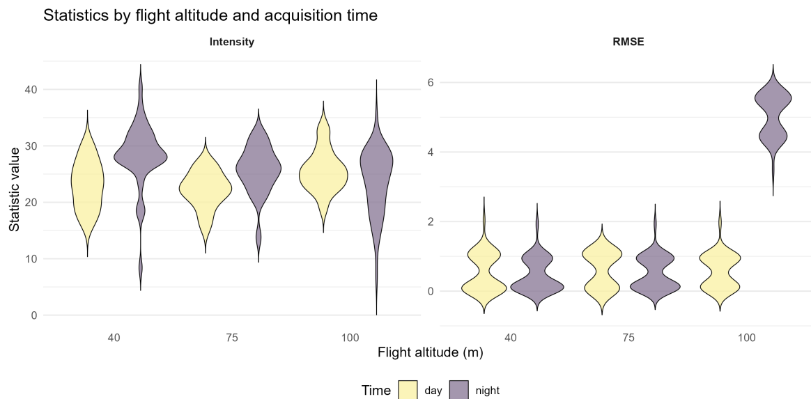
Figure 2: Open treed metrics
