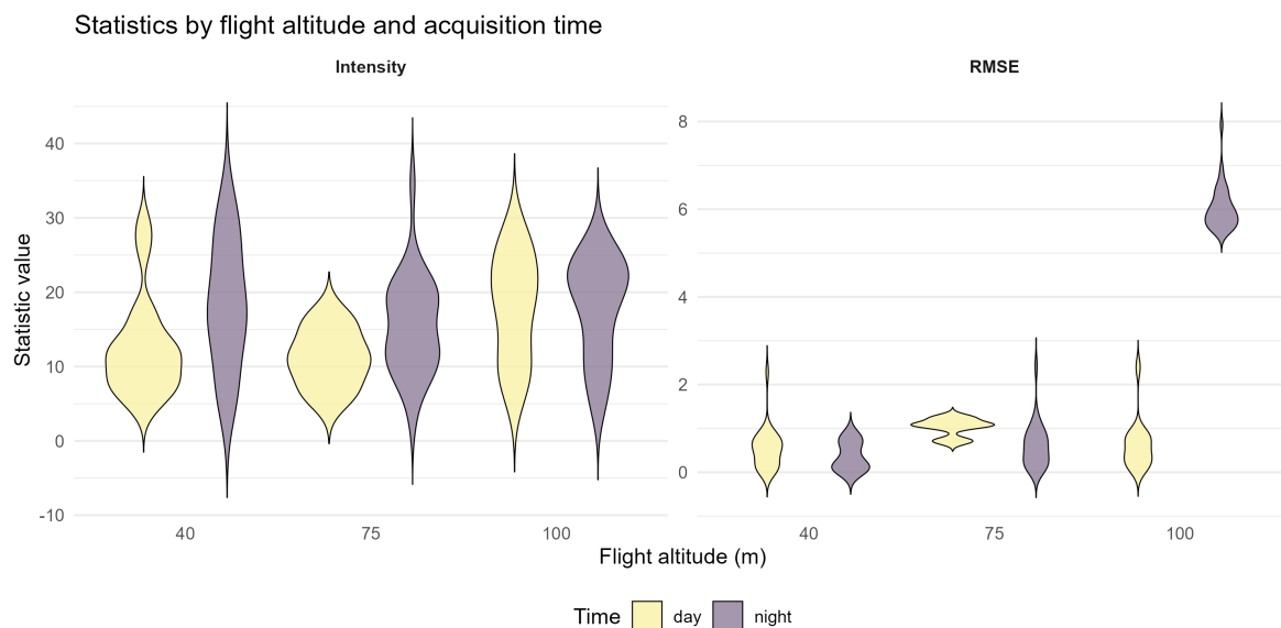
Figure 3: Dense treed metrics
