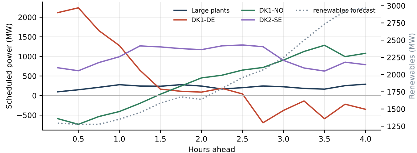
Optimised dispatch trajectory
