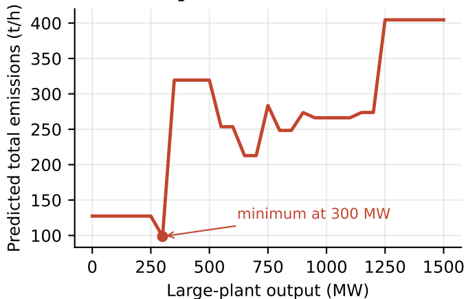
Original: unconstrained tree
