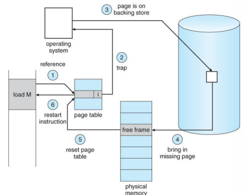
Figura 14.6: Page fault
