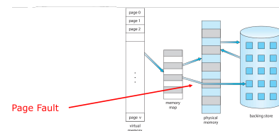
Figura 14.5: Page fault
