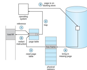
Figura 14.4: Page fault
