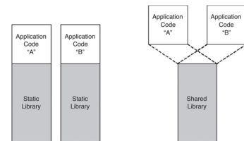
Figura 14.1: File .dll
