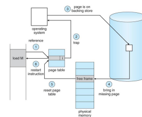
Figura 8.5: Page fault
