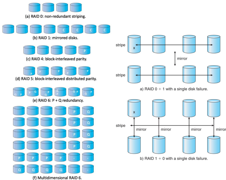
Figura 11.4: Schemi RAID
