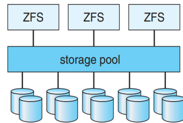
Figura 11.6: ZFS e storage a pool
