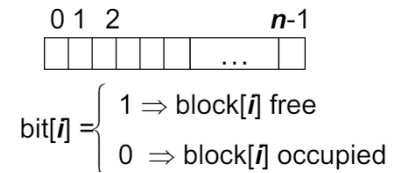
Figura 20.4: bit map
