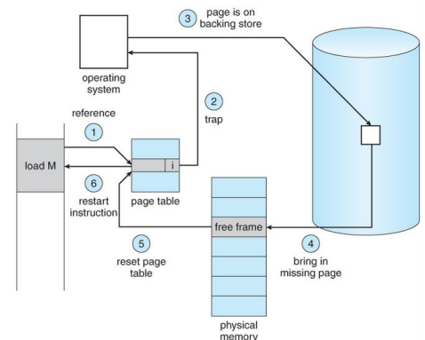
Figura 15.6: Page fault
