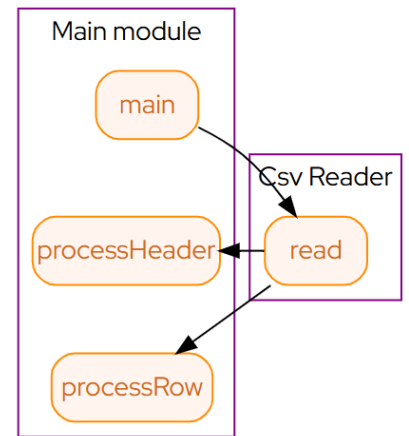
Figure 7.2: Call diagram
