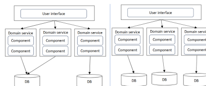
Figure 15.3: DB options
