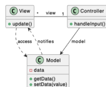
Figure 2.1: MVC
