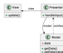
Figure 2.2: MVP
