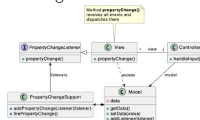
Figure 2.1: MVC
