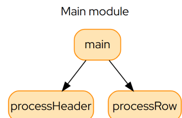
Figura 7.1: Call diagram
