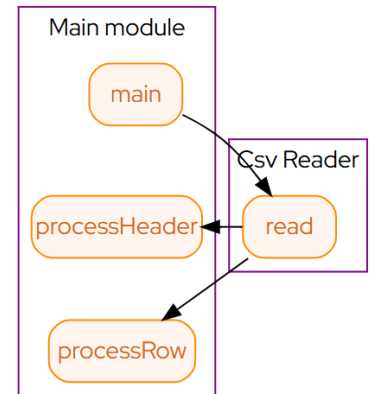
Figura 7.2: Call diagram
