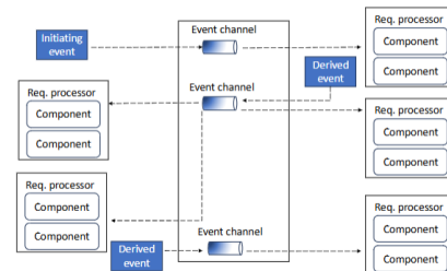
Figura 15.7: Fire and forget
