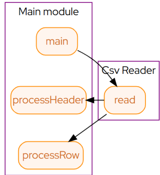
Figura 7.2: Call diagram
