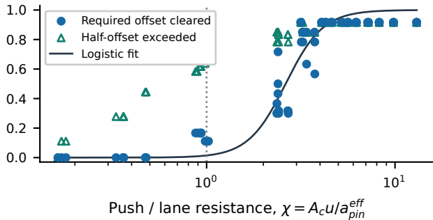
(a) Transition in lateral clearance
