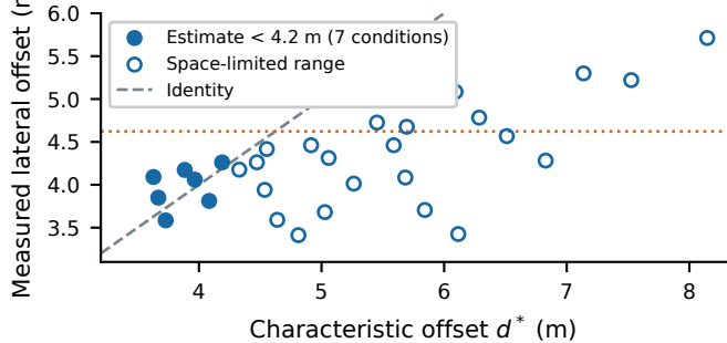
(b) Width estimate and road limitation
