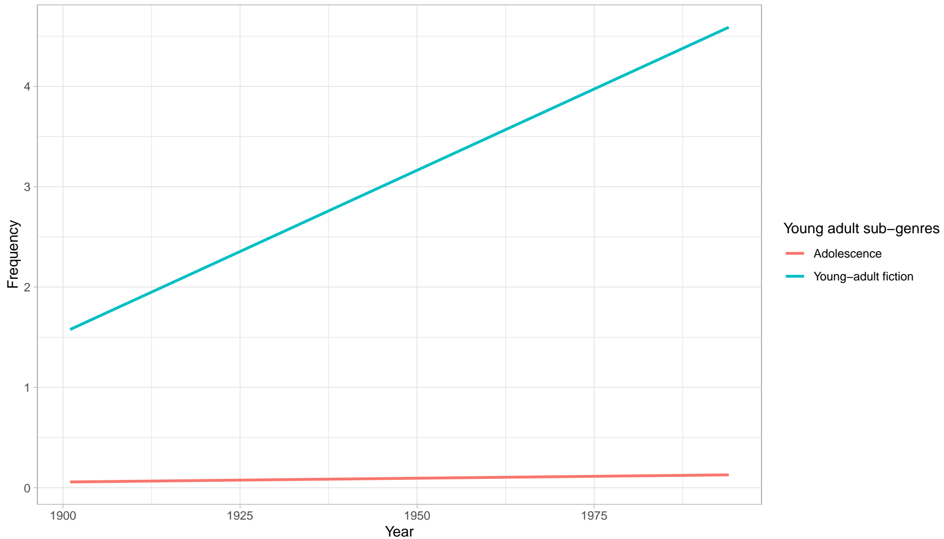
Breakdown of absolute occurrence of young adult sub-genres
