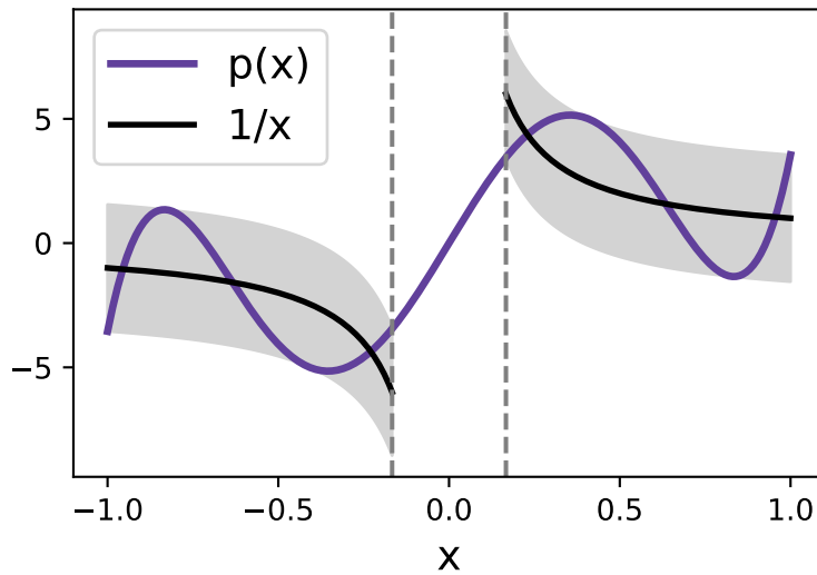
d=5, \varepsilon \approx 2.6
