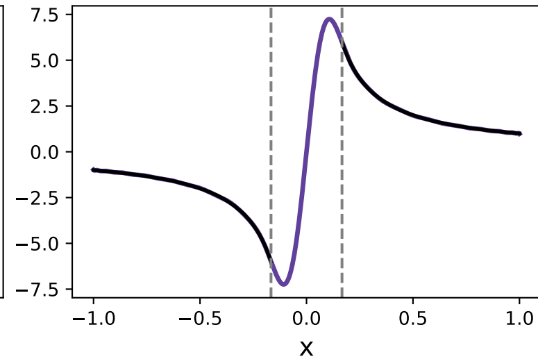
d=35, \varepsilon \approx 0.016
