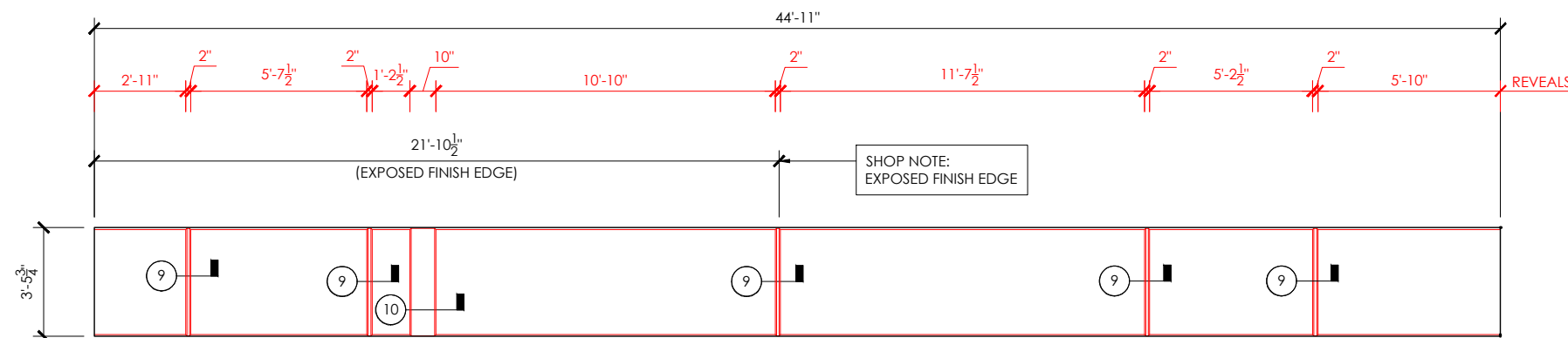
REVEAL DRAWING
