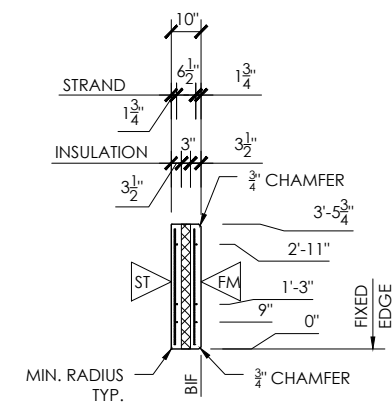
SECTION VIEW
