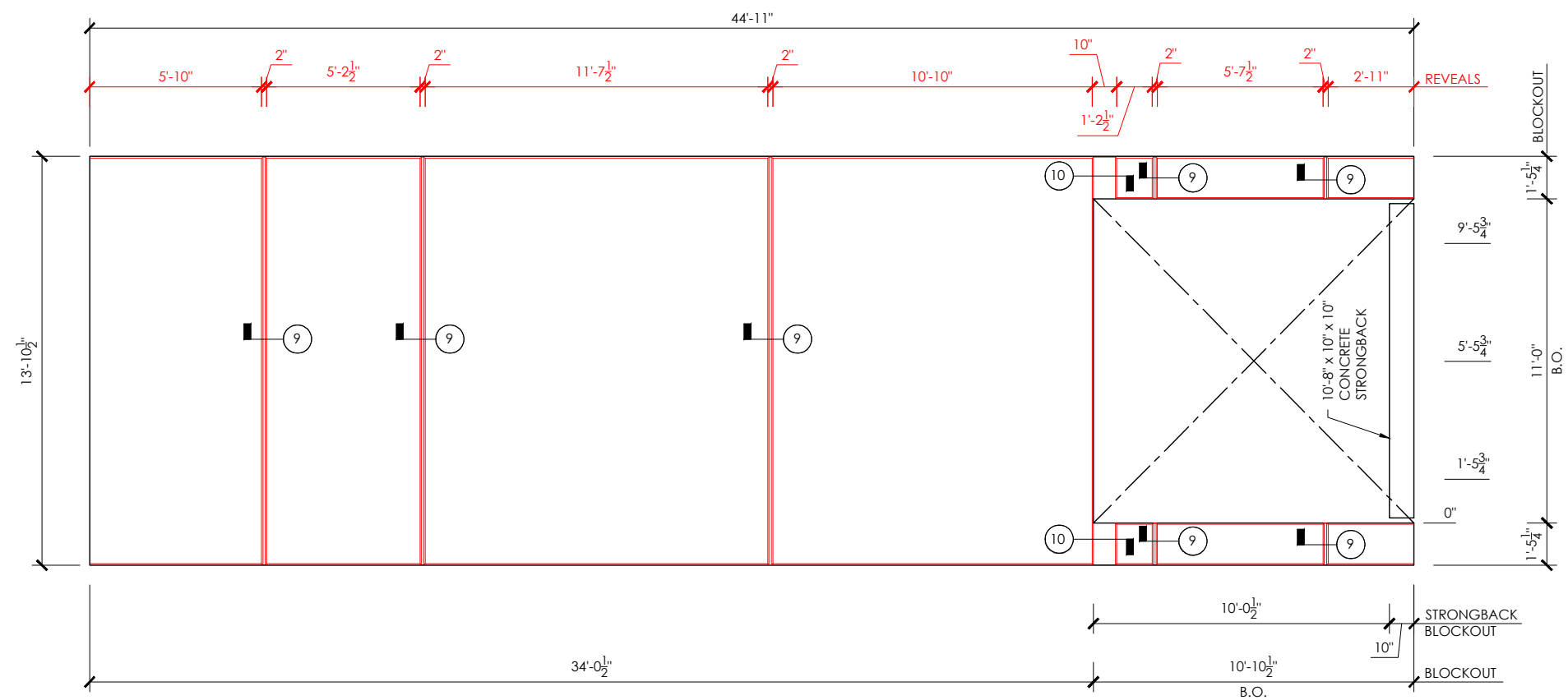
REVEAL DRAWING
