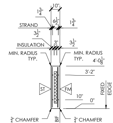
SECTION VIEW
