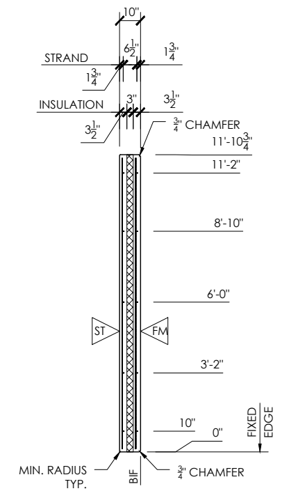
SECTION VIEW
