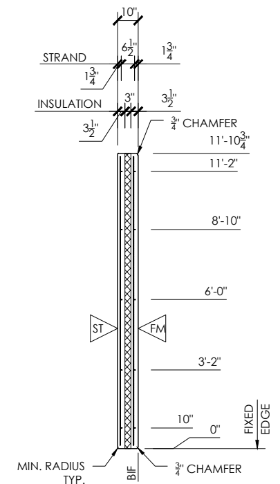
SECTION VIEW
