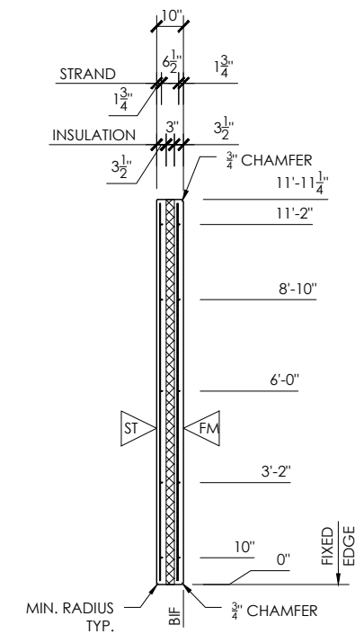
SECTION VIEW
