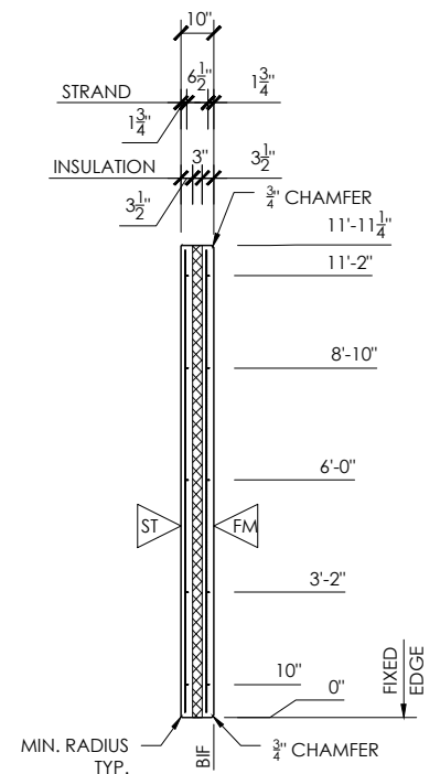
SECTION VIEW
