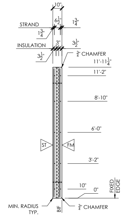
SECTION VIEW
