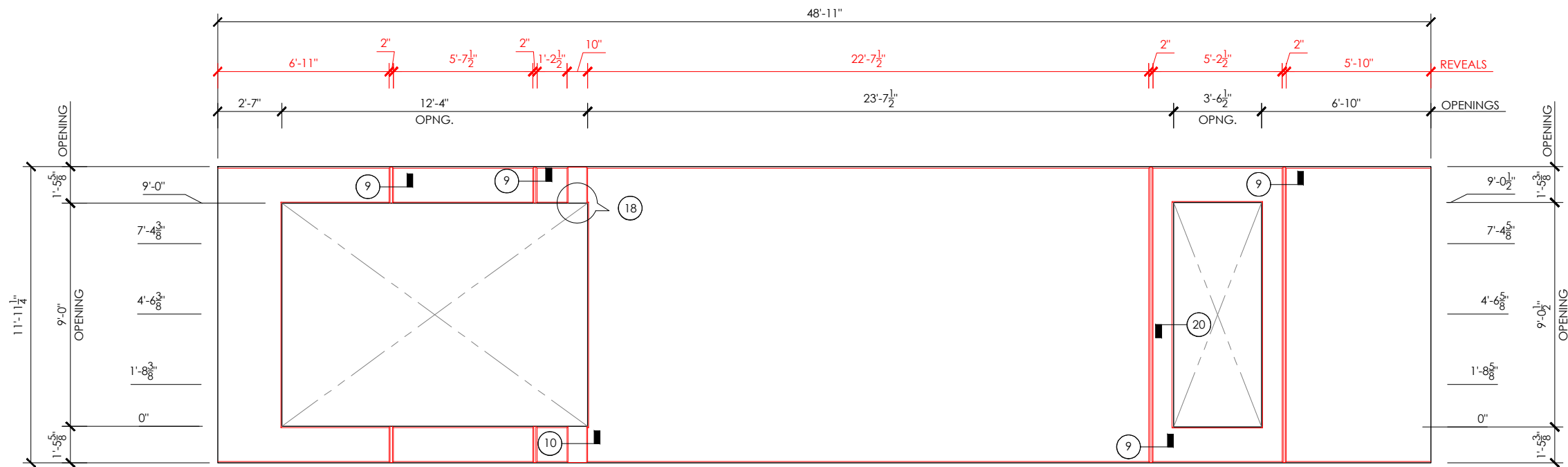
REVEAL DRAWING
