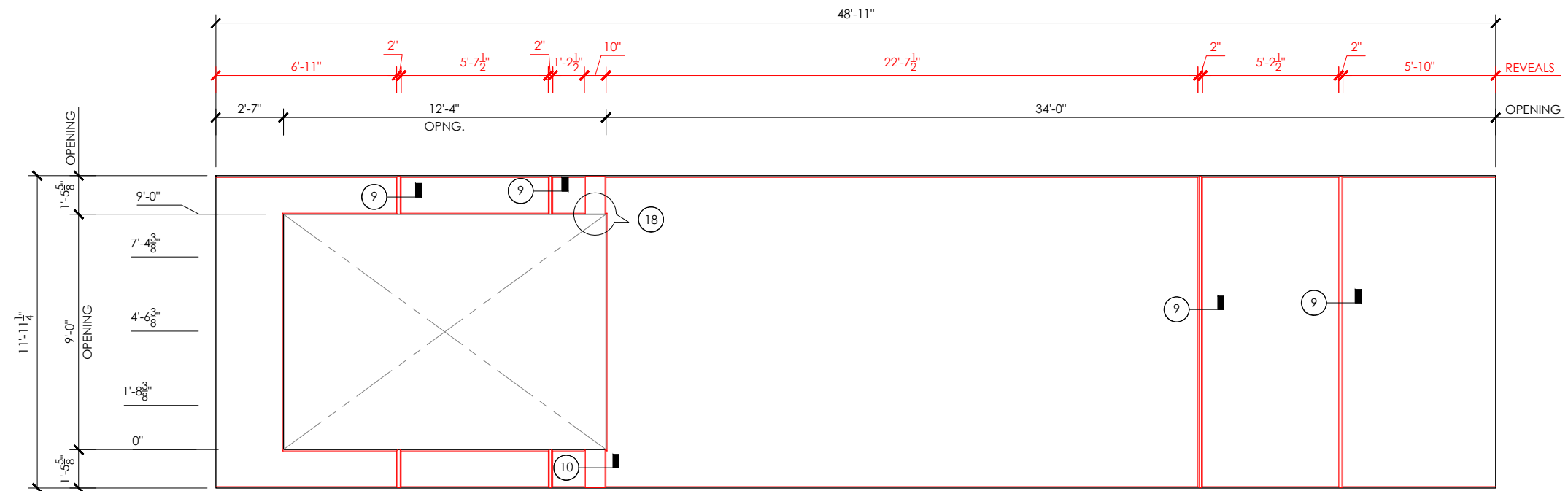
REVEAL DRAWING
