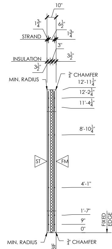
SECTION VIEW
