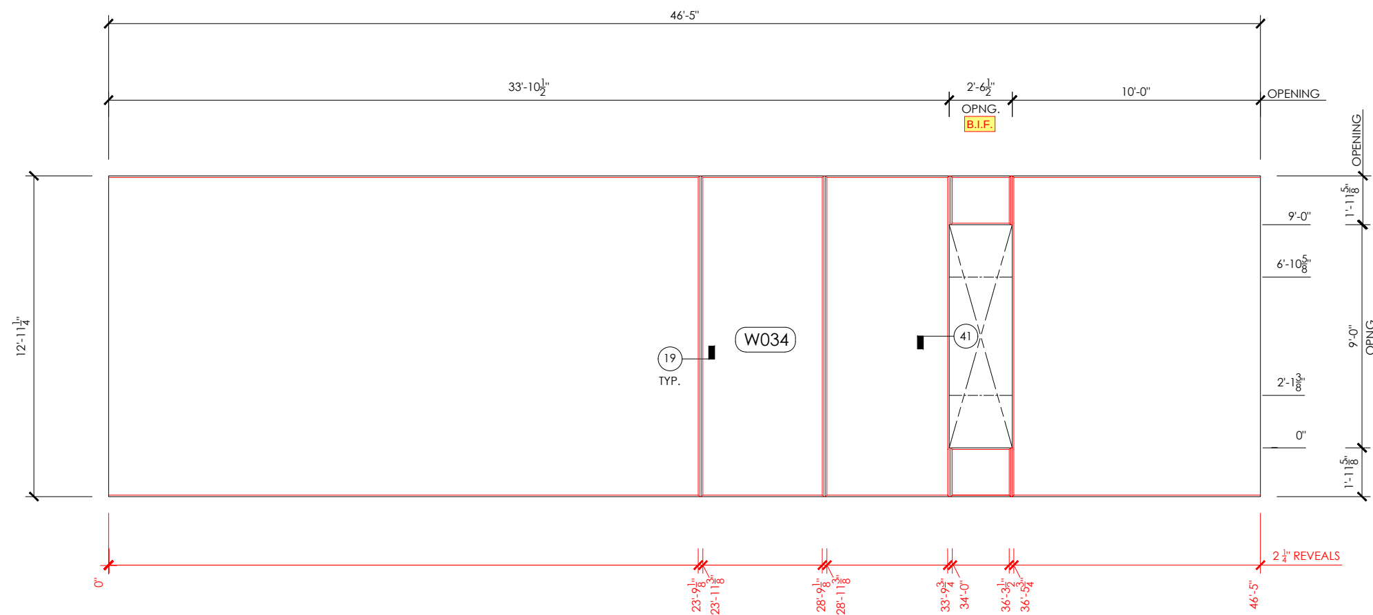
REVEAL DRAWING
