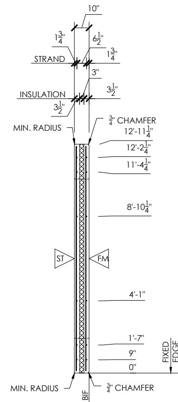
SECTION VIEW
