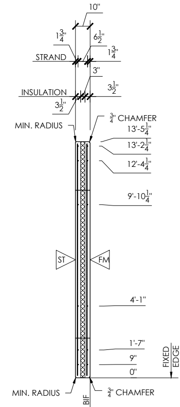
SECTION VIEW
