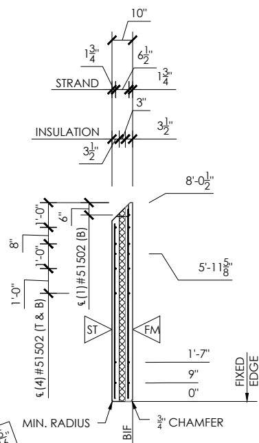
SECTION VIEW
