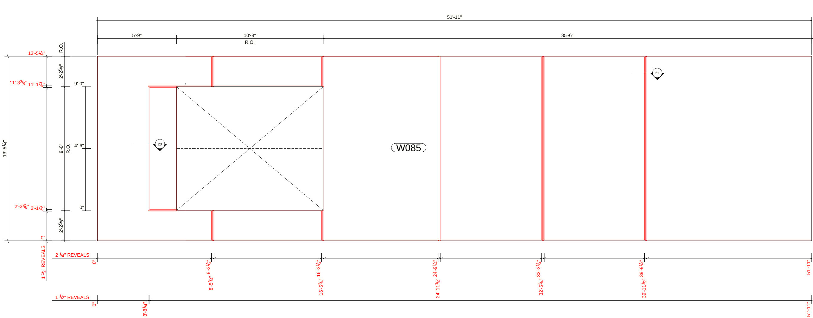
REVEAL DRAWING
