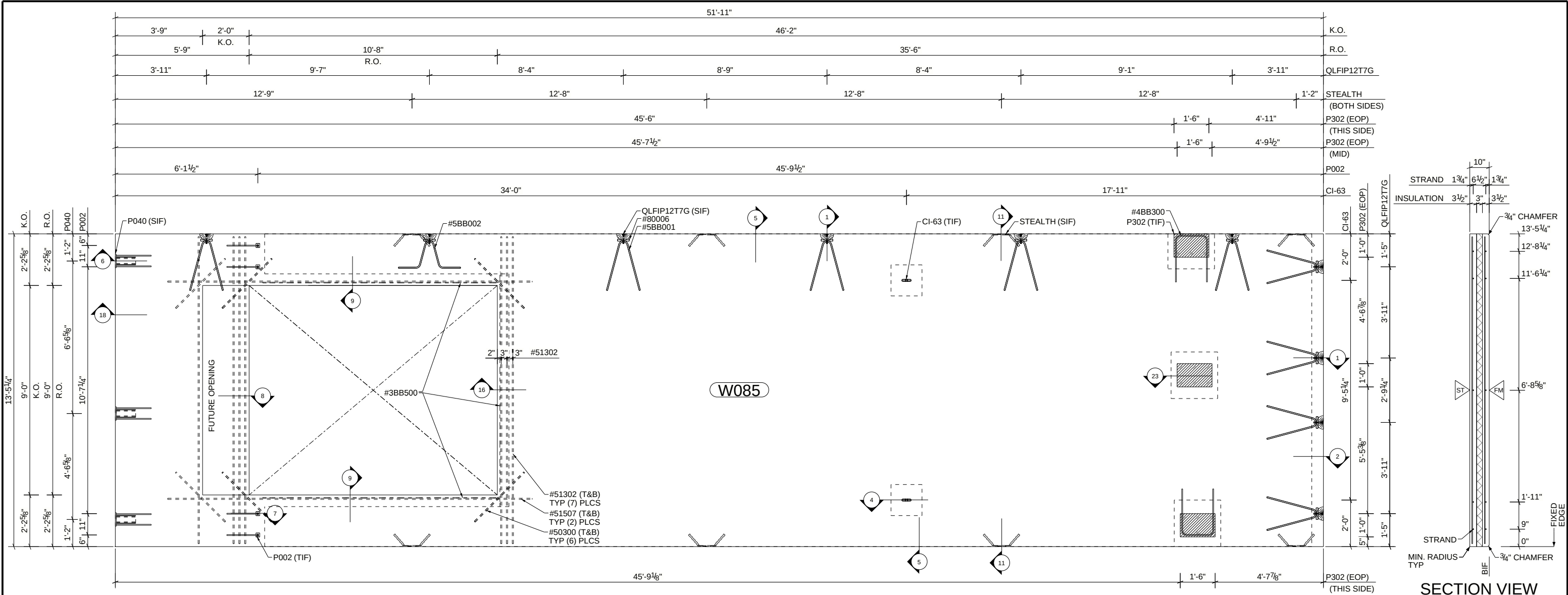
FORM VIEW
