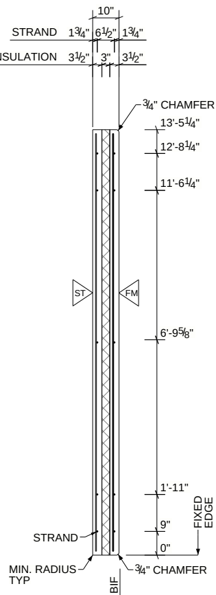
SECTION VIEW
