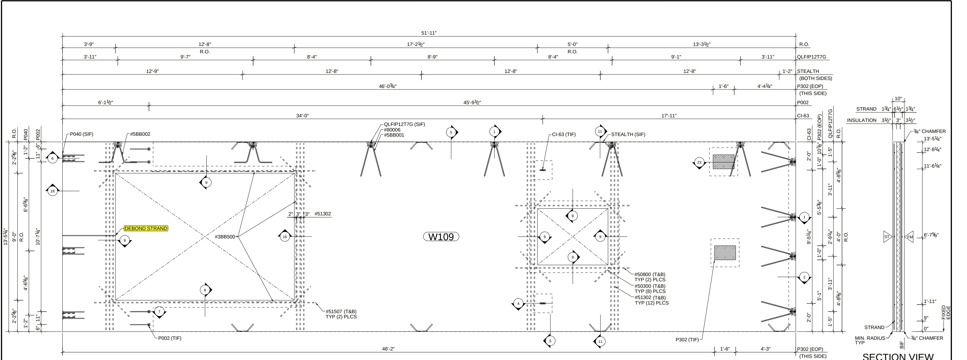
FORM VIEW
