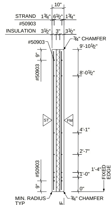
SECTION VIEW
