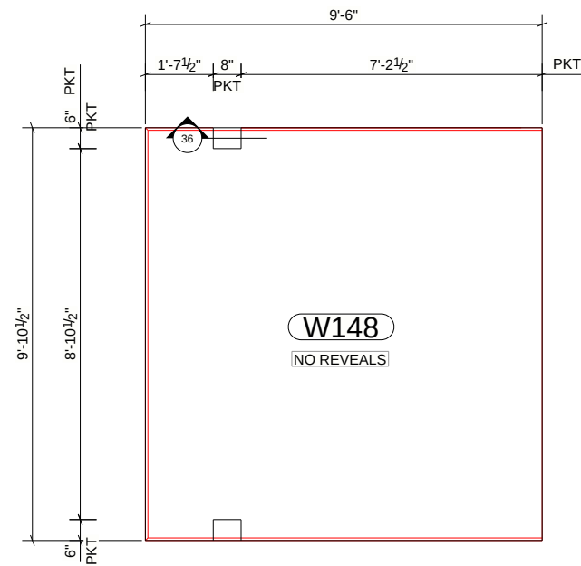
REVEAL DRAWING
