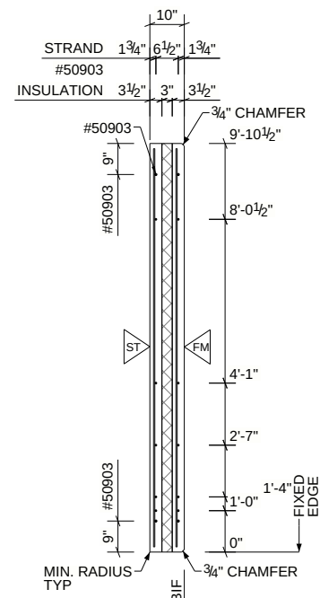
SECTION VIEW
