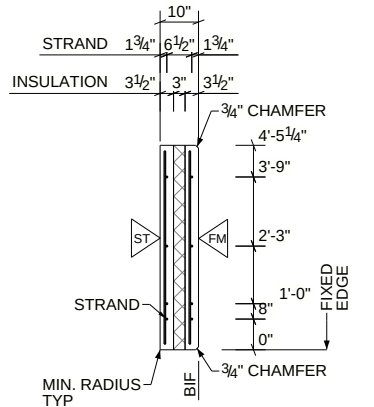
SECTION VIEW
