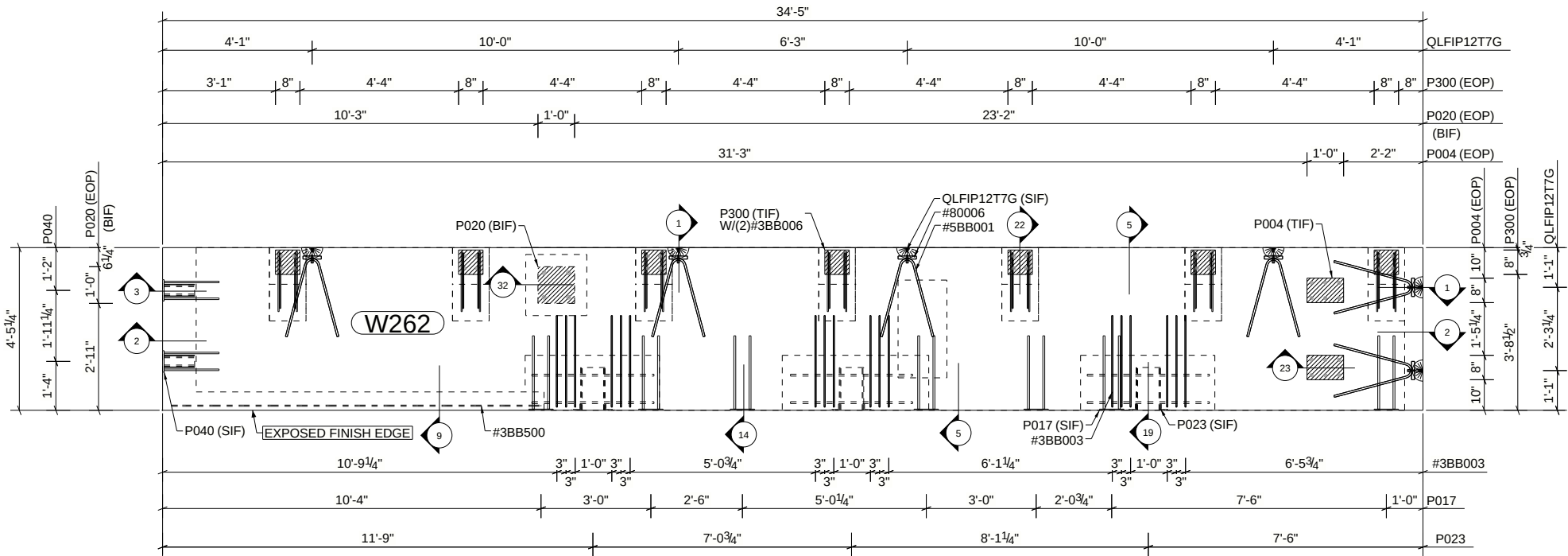
FORM VIEW
