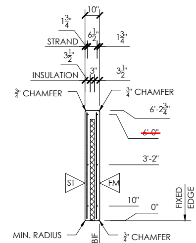
SECTION VIEW
