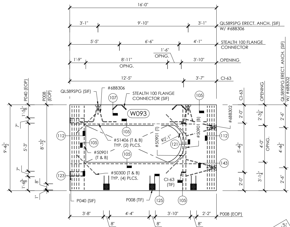
FORM VIEW
