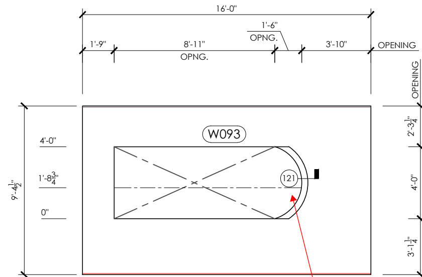
REVEAL DRAWING
