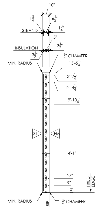
SECTION VIEW
