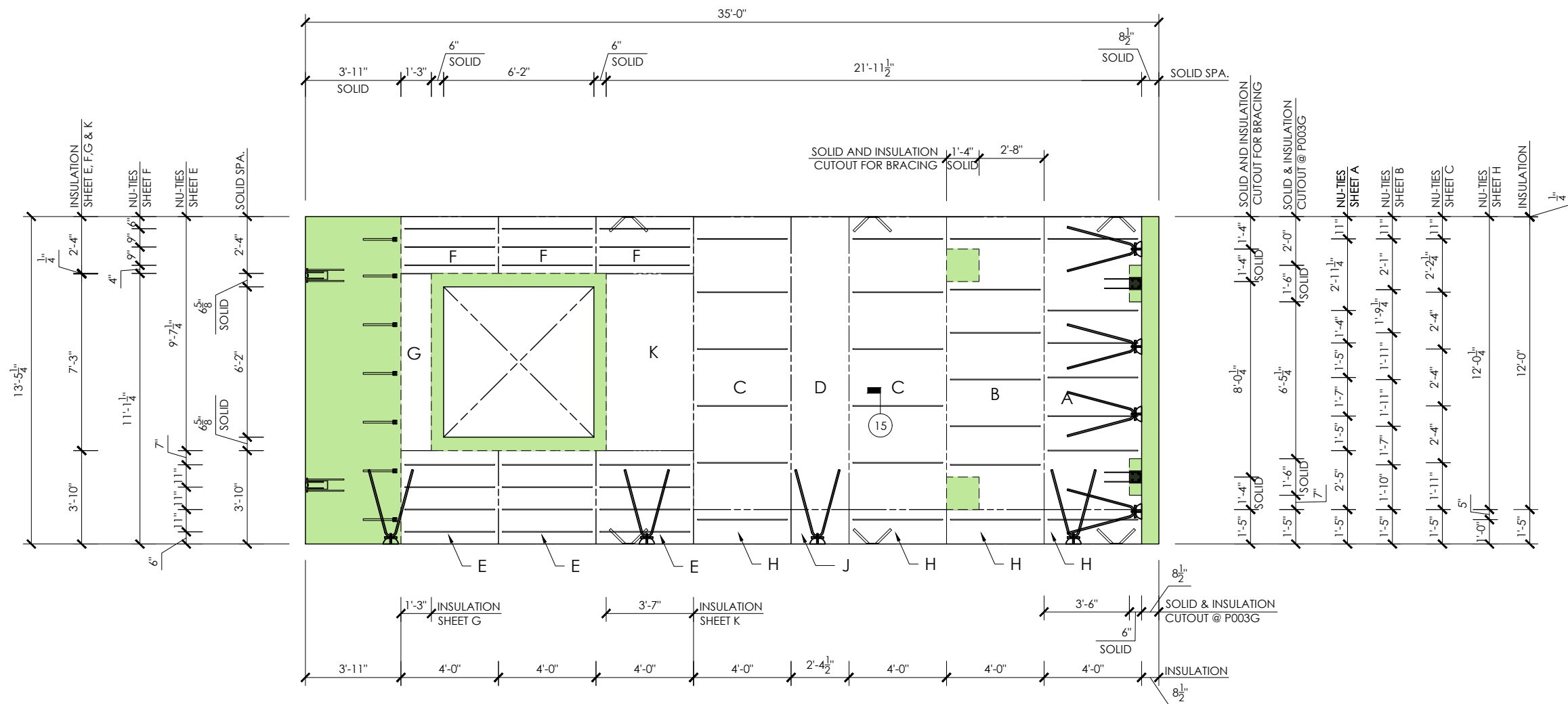
FOAM DRAWING
