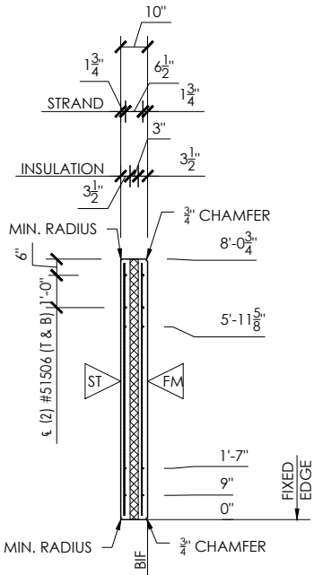
SECTION VIEW
