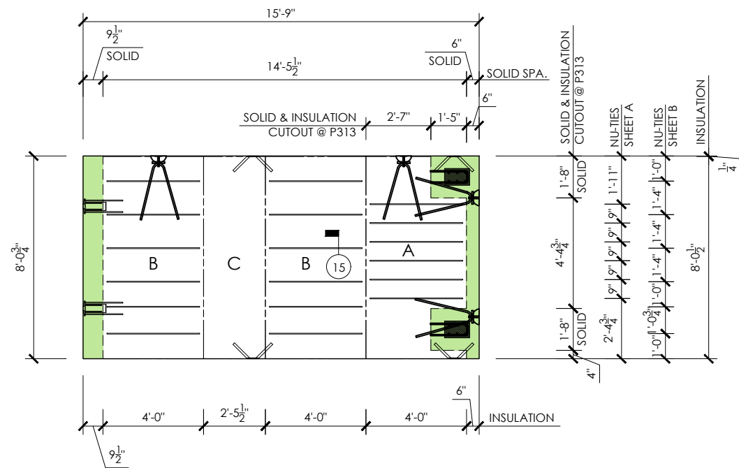
FOAM DRAWING
