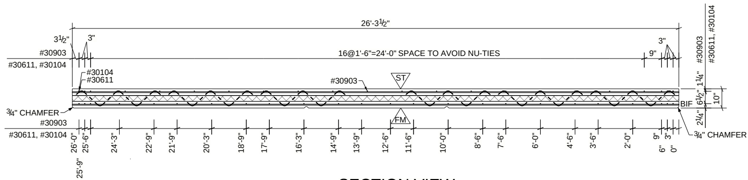
SECTION VIEW
