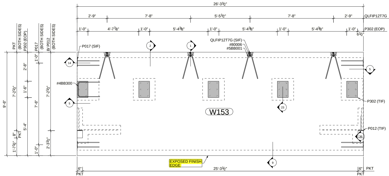
FORM VIEW
