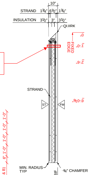
SECTION VIEW
