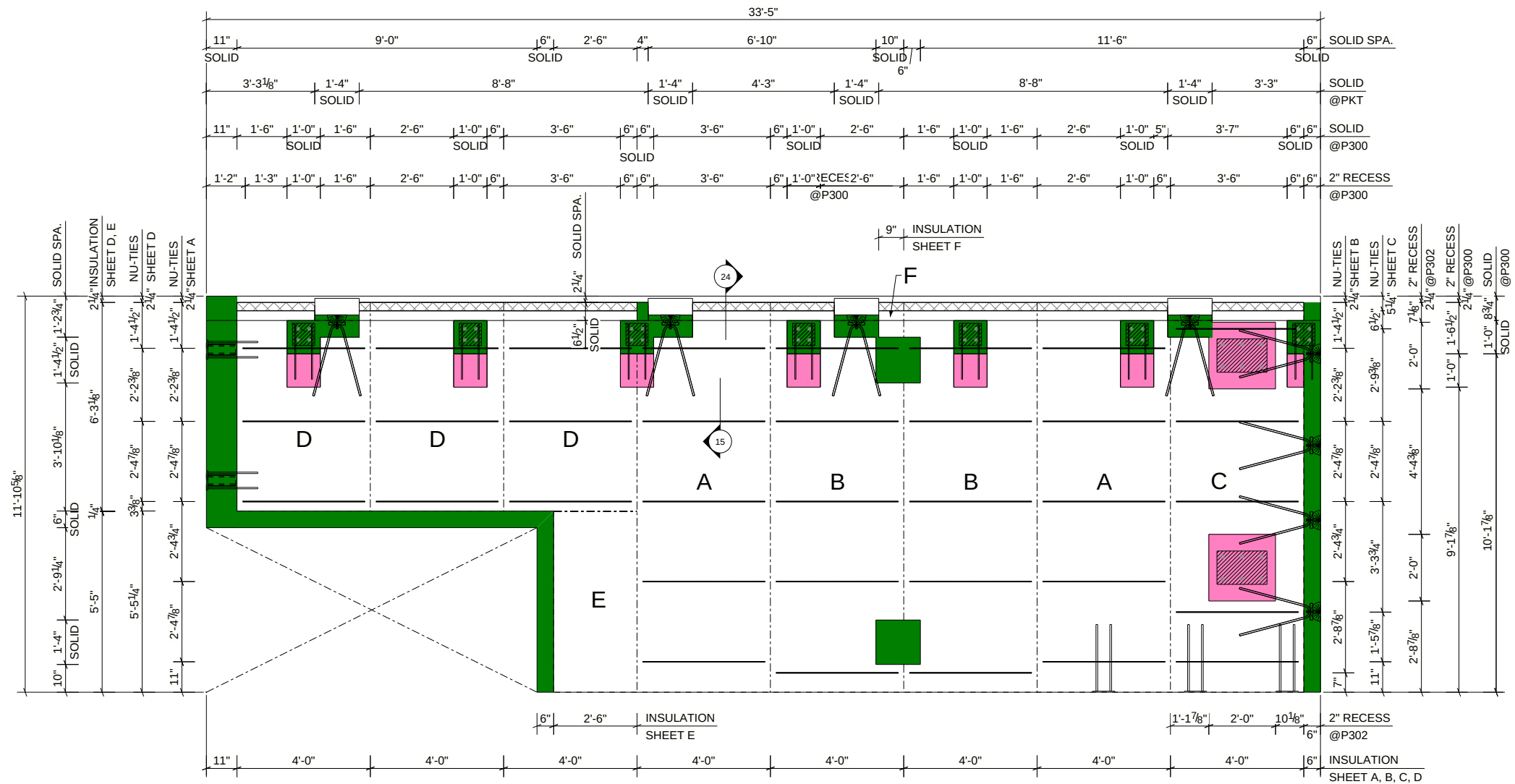
FOAM DRAWING
