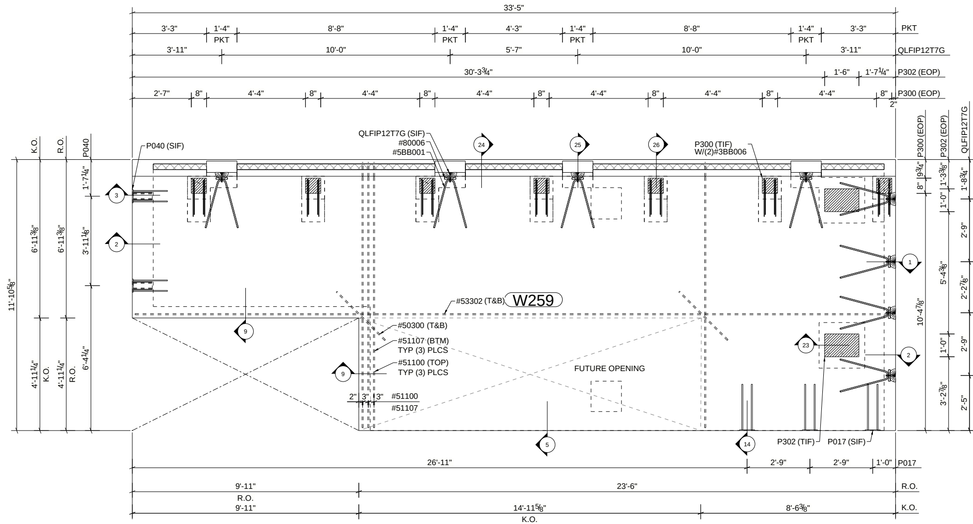
FORM VIEW
