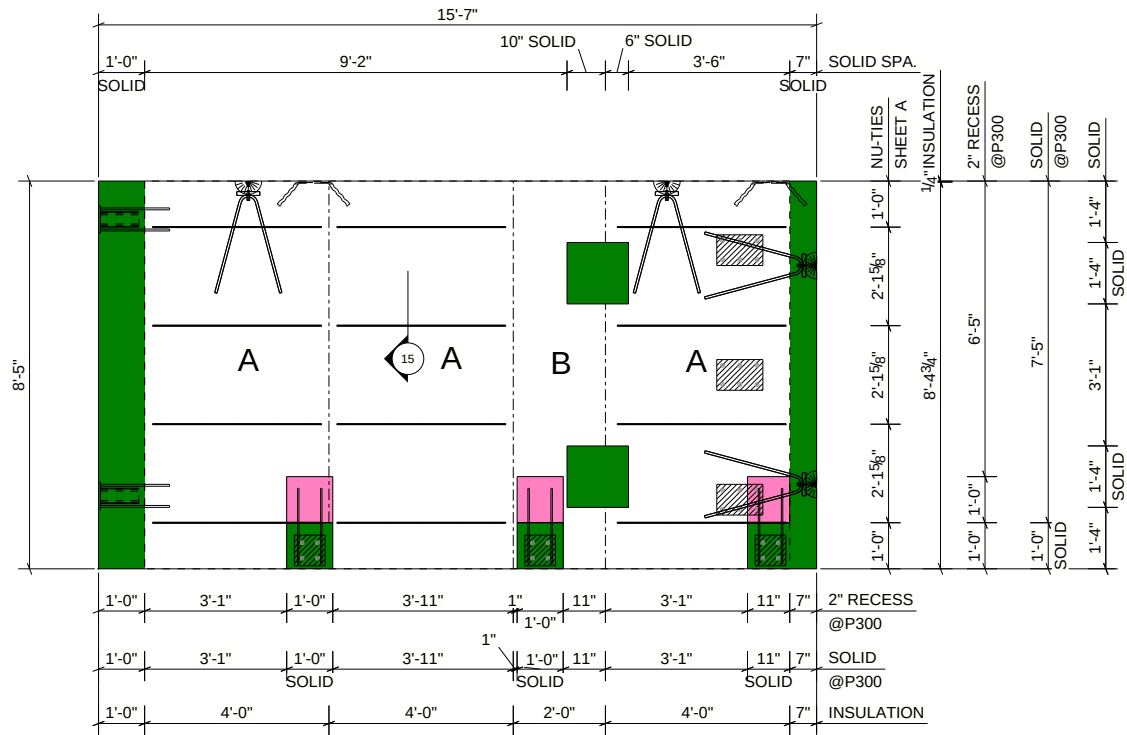
FOAM DRAWING
