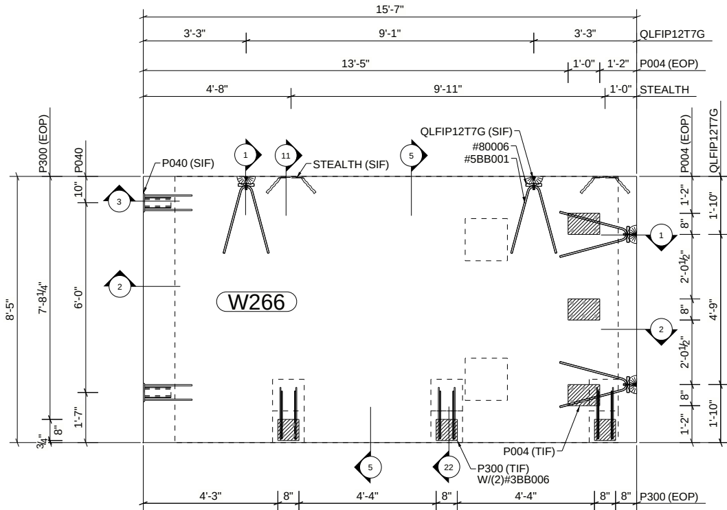
FORM VIEW
