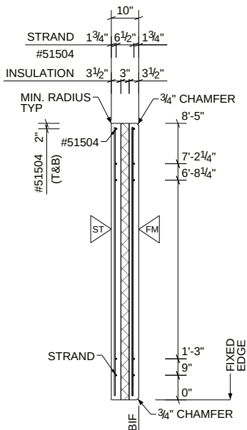
SECTION VIEW
