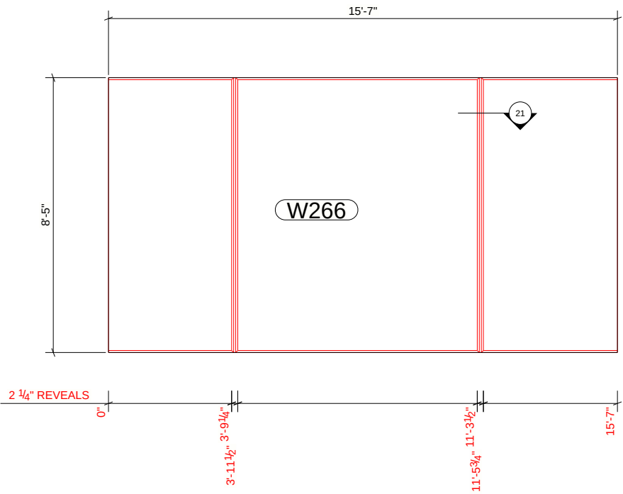
REVEAL DRAWING
