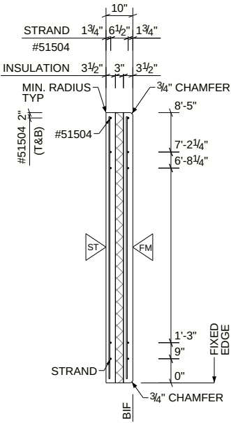
SECTION VIEW
