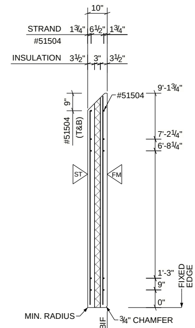
SECTION VIEW
