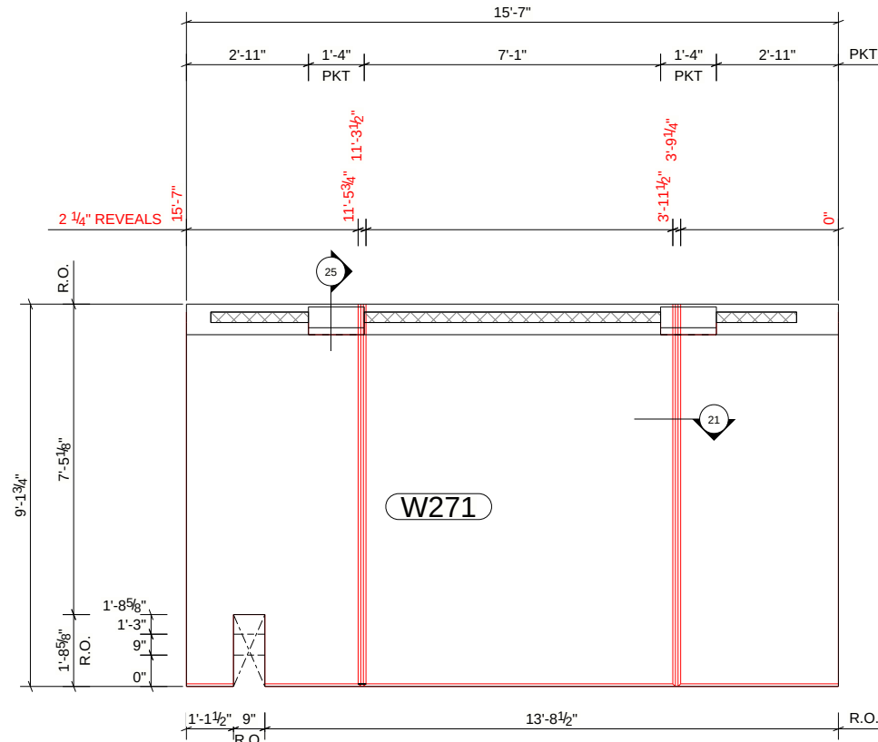
REVEAL DRAWING
