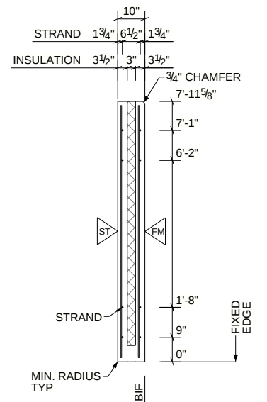
SECTION VIEW
