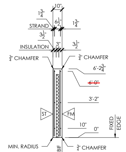
SECTION VIEW
