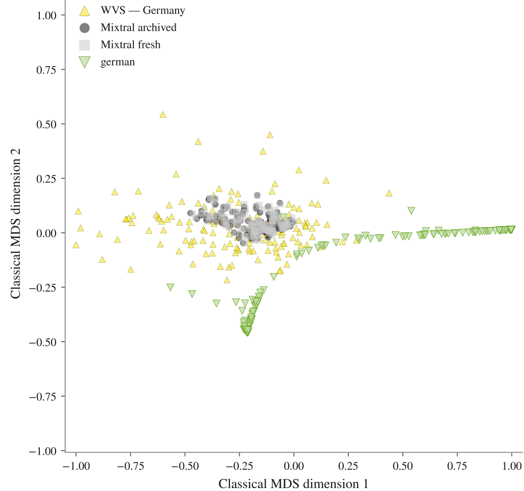
NTP · 141 subpopulations · mean nEMD Mixtral archived 0.061, Mixtral fresh 0.062, german 0.182
