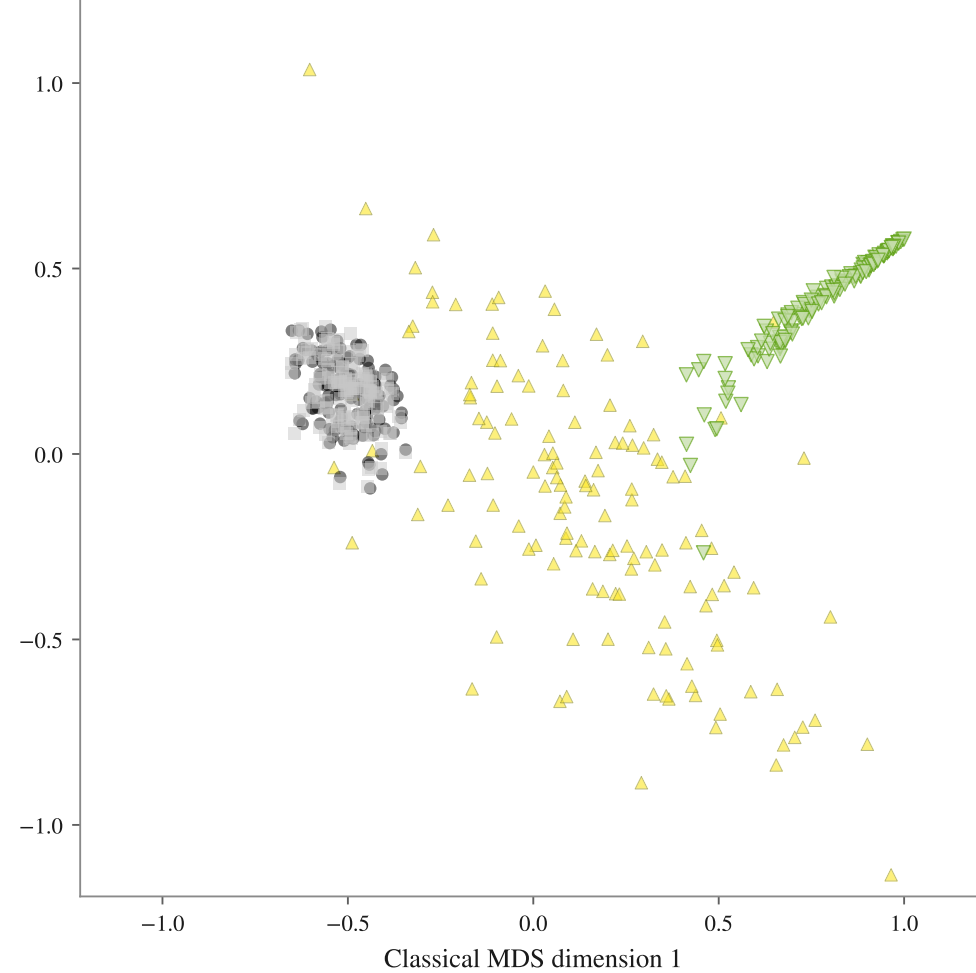
NTP · 139 subpopulations · mean nEMD Mixtral archived 0.098, Mixtral fresh 0.098, german 0.114
