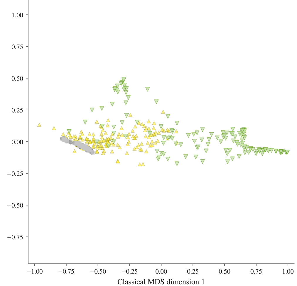
NTP · 141 subpopulations · mean nEMD Mixtral archived 0.155, Mixtral fresh 0.155, german 0.378
