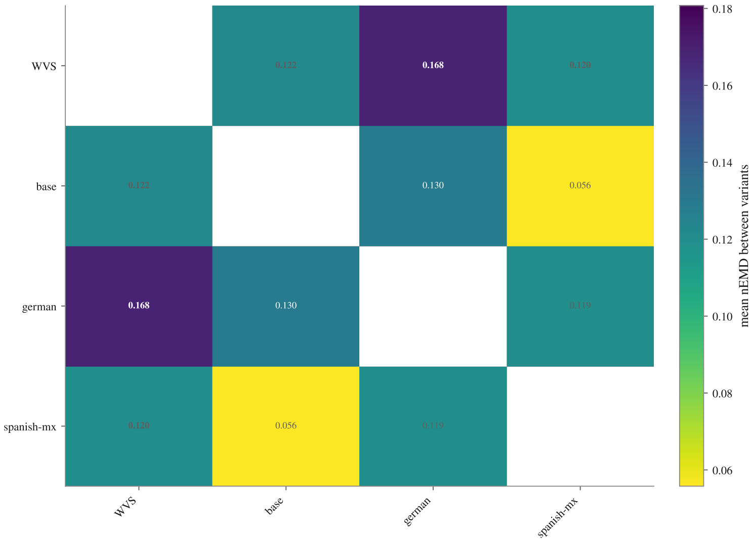
All models
