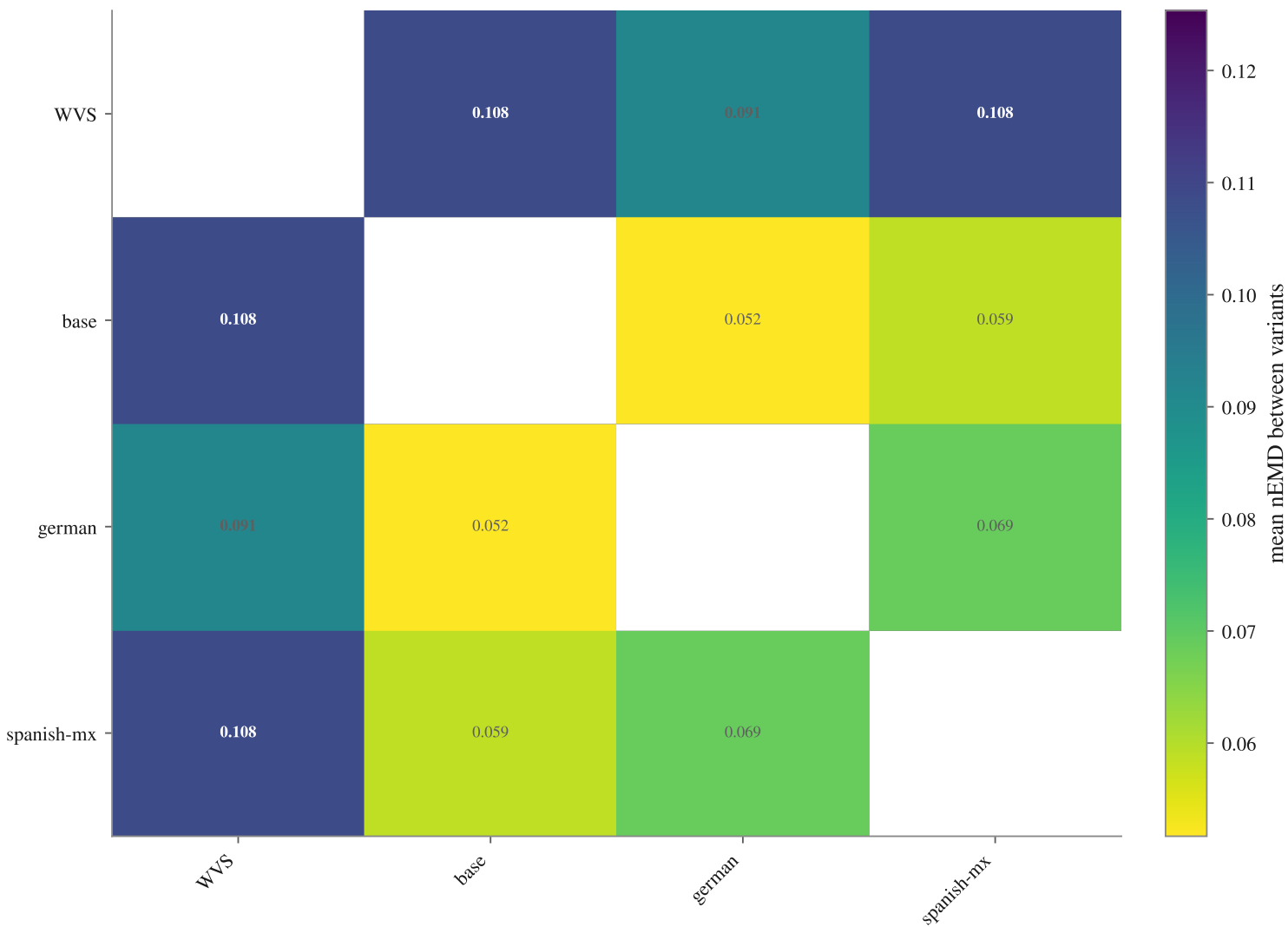
Muse-Glimmer-30B
