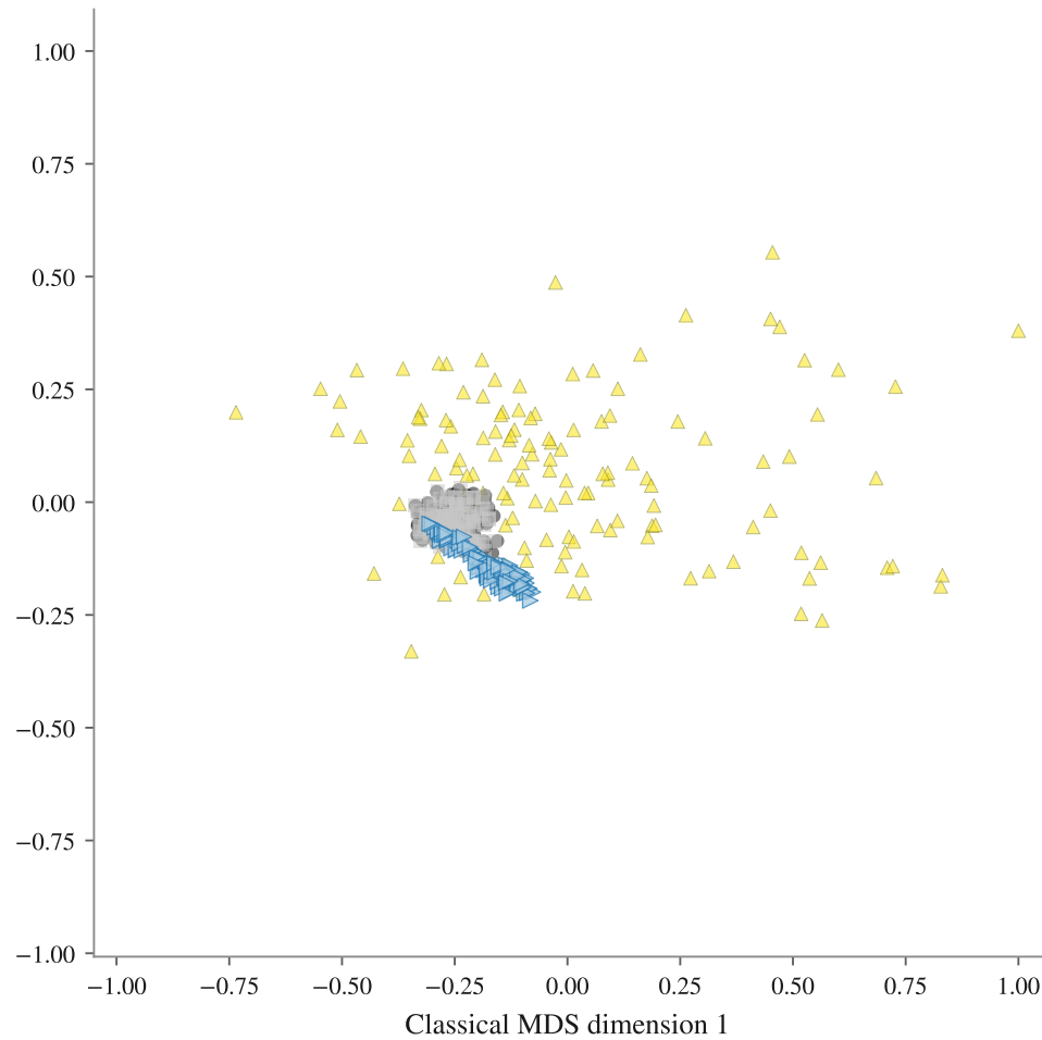
NTP · 131 subpopulations · mean nEMD Mixtral archived 0.099, Mixtral fresh 0.099, spanish-mx 0.107
