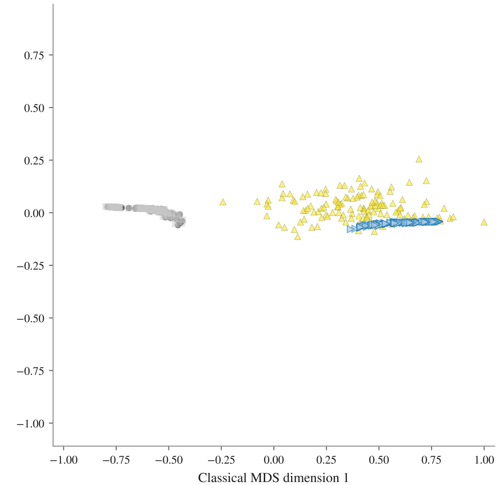
NTP · 131 subpopulations · mean nEMD Mixtral archived 0.404, Mixtral fresh 0.406, spanish-mx 0.129
