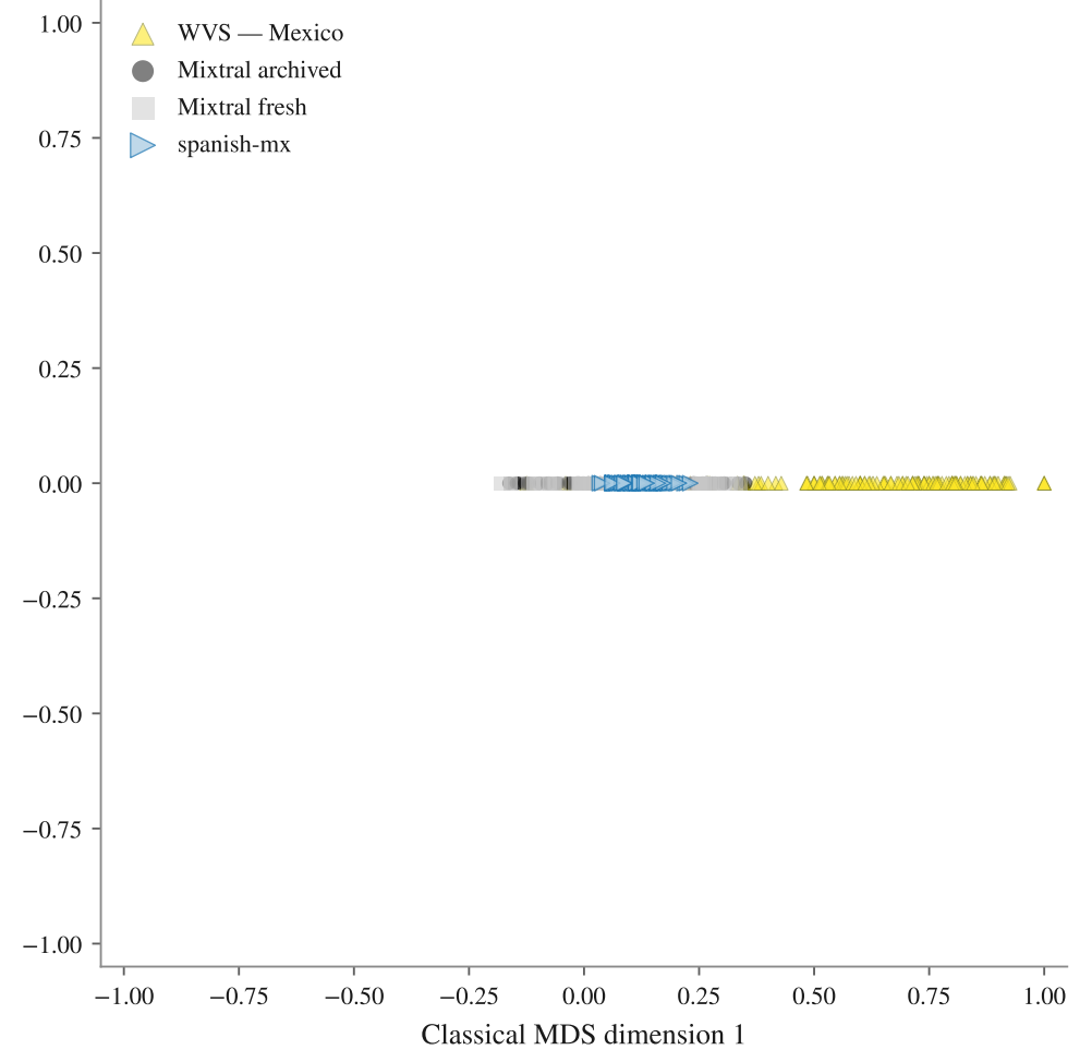
FA · 131 subpopulations · mean nEMD Mixtral archived 0.442, Mixtral fresh 0.282, spanish-mx 0.390
