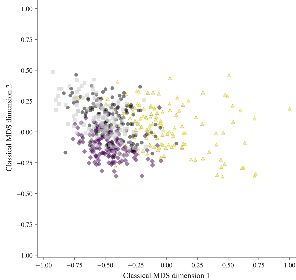
FA · 131 subpopulations · mean nEMD base 0.142, Mixtral archived 0.132, Mixtral fresh 0.149
