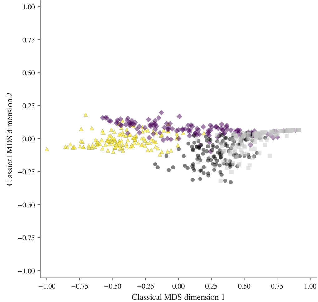
FA · 131 subpopulations · mean nEMD base 0.243, Mixtral archived 0.312, Mixtral fresh 0.428
